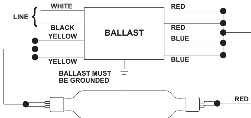
Wiring Diagram 1
